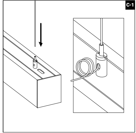
C-1. Fixing the Suspension Cable to the Rear Capsule of the Luminaire
